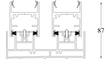
SILL VISIBLE WIDTH
