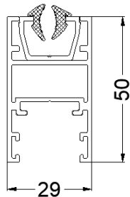
SHUTTER AT INTERLOCK
