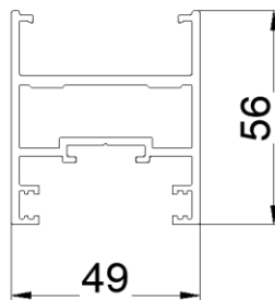
SHUTTER AT HANDLE SECTION
