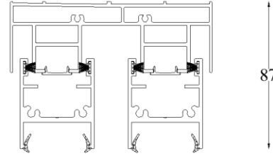
HEAD VISIBLE WIDTH
