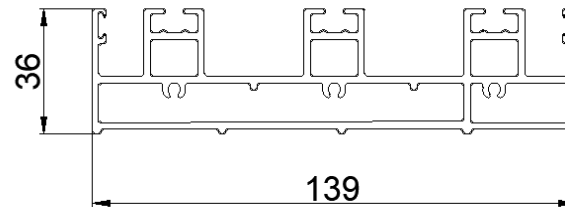
3-TRACK
