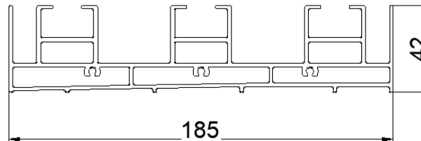
3-TRACK
