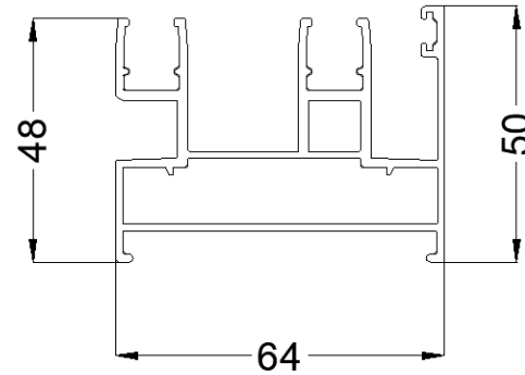
2-TRACK
