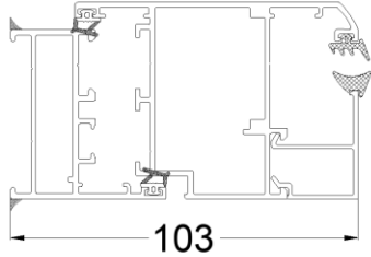
VISIBLE WIDTH ALL 4 SIDES
