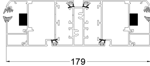
DOUBLE OPENABLE WITH FIXED MULLION
