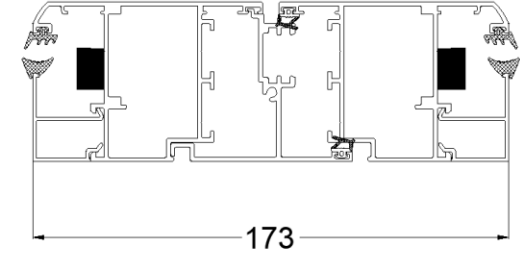
FRENCH WINDOW WITH FLY MULLION
