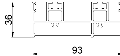
2-TRACK
