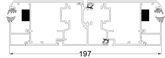
FRENCH WINDOW WITH FLY MULLION
