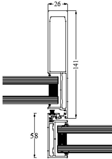
SHUTTER AT INTERLOCK
