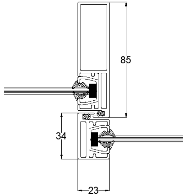
SHUTTER AT INTERLOCK
