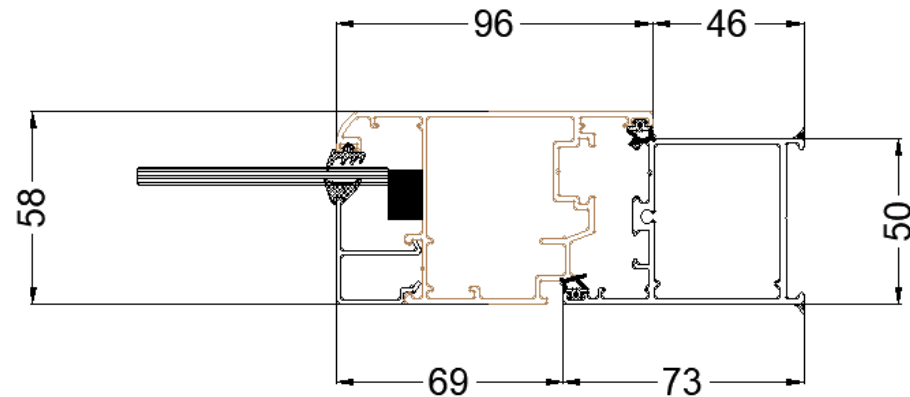
FRAME SHUTTER CONNECTION SIDES
