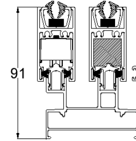
SILL VISIBLE WIDTH
