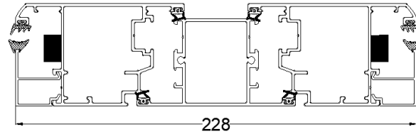
DOUBLE OPENABLE WITH FIXED MULLION
