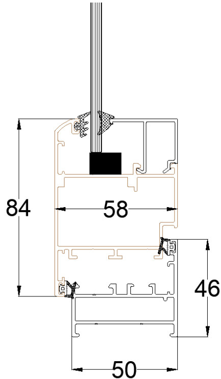
FRAME SHUTTER CONNECTION
