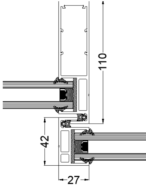
SHUTTER AT INTERLOCK
