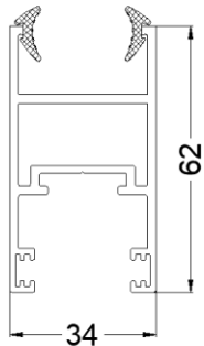
SHUTTER AT HANDLE SECTION
