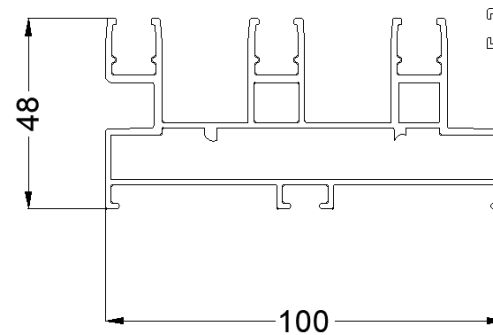
3-TRACK
